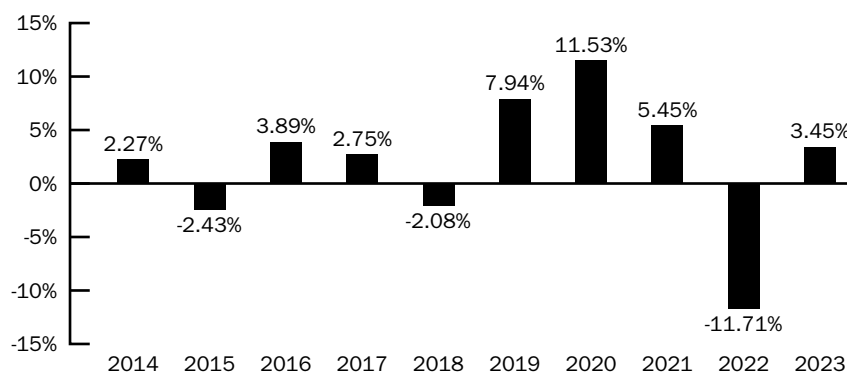
Investor A Shares ANNUAL TOTAL RETURNS Inflation Protected Bond Portfolio As of 12/31
